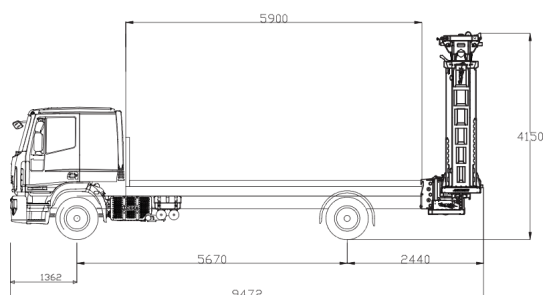
Blade TMA mounted to the IVECO Eurocargo
